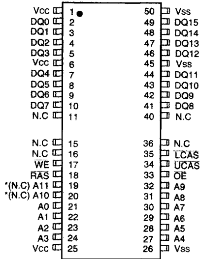
44/50Pin Plastic TSOP- II (400mil)
