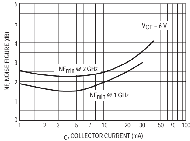
Figure 7. Minimum Noise Figure versus Collector Current
