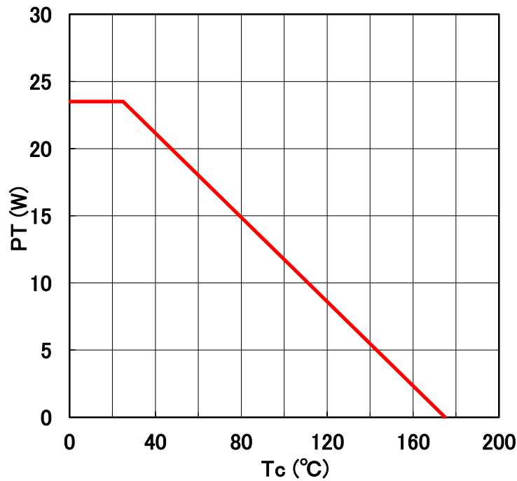
Power Dissipation vs. Case Temperature
