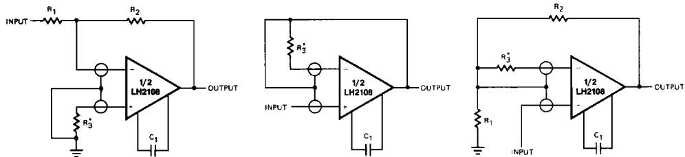
INVERTING AMPLIFIER
