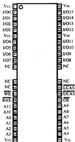
44(50) TSOP II
