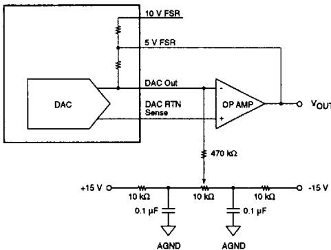
Figure 4 - Offset Compensation
