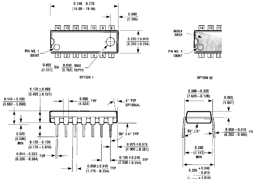
14-Lead Molded Dual-In-Line Package (N) Order Number DM74LS40N NS Package Number N14A
