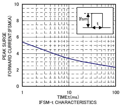
IFSM-t CHARACTERISTICS
