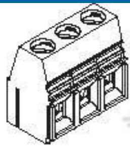
TE Part #1-1986660-3 3 Posn Power Connector, Black, 10.16 mm
