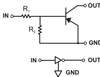
SCHEMATIC DIAGRAM
