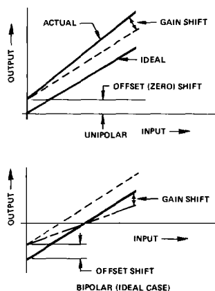
Figure 3. Unipolar and Bipolar Drifts
