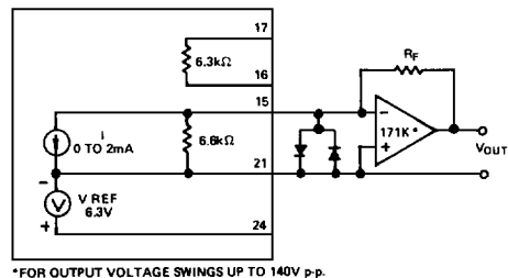
Figure 13. External Op Amp—Using External Feedback Resistors
