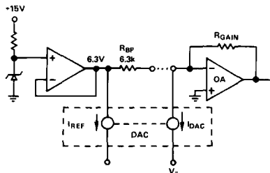
Figure 2. Bipolar Configuration
