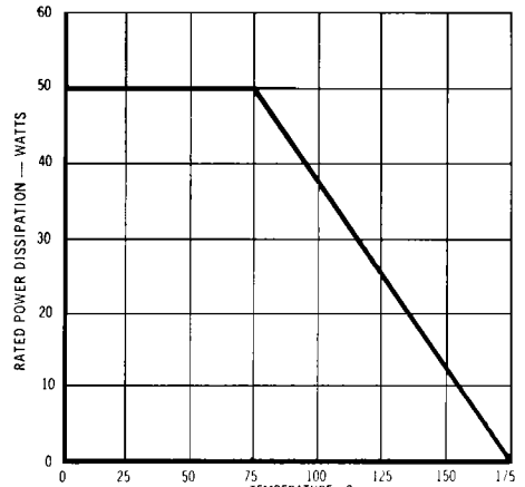
FIGURE 2 POWER DERATING CURVE
