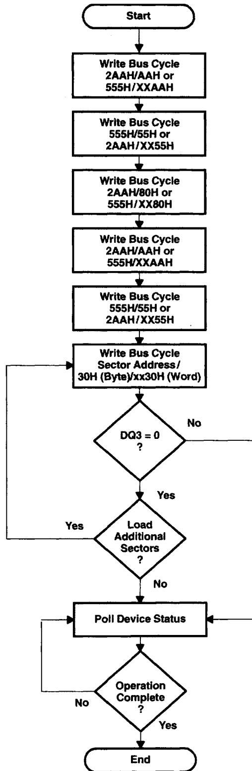
Figure 14. Sector-Erase Algorithm
