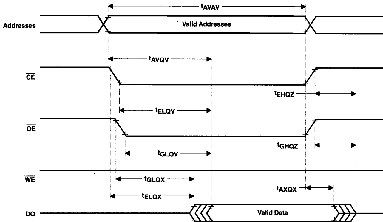
Figure 8. AC Waveform for Read Operation
