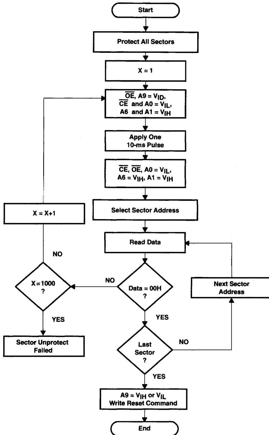
Figure 22. Sector-Unprotect Algorithm
