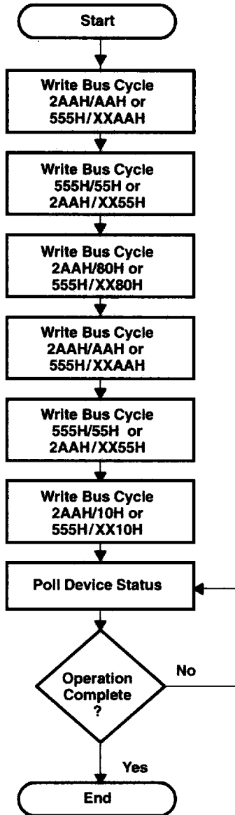
Figure 12. Chip-Erase Algorithm
