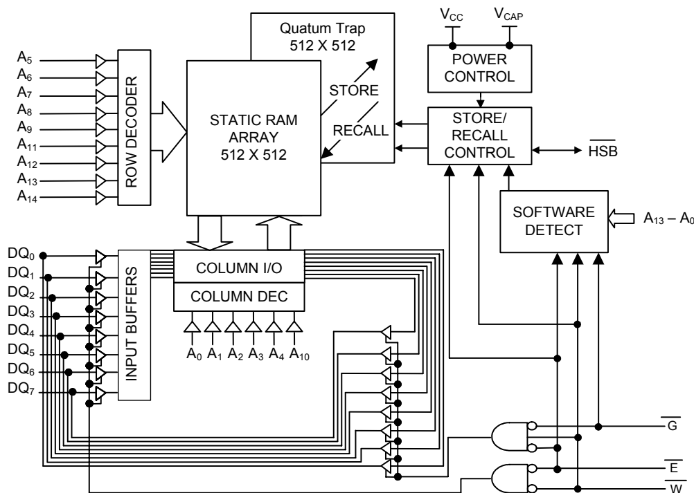
Figure 1. Block Diagram
