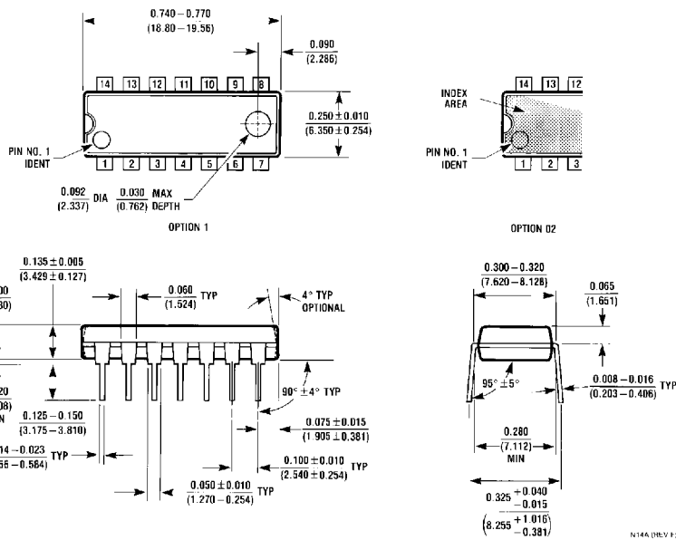
14 Lead Plastic Dual-In-Line Package (P) NS Package Number N14A
