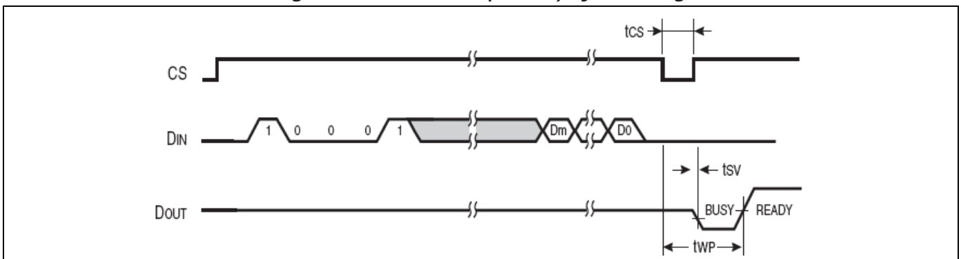
Figure 5.10-5. Write All (WRALL) Cycle Timing
