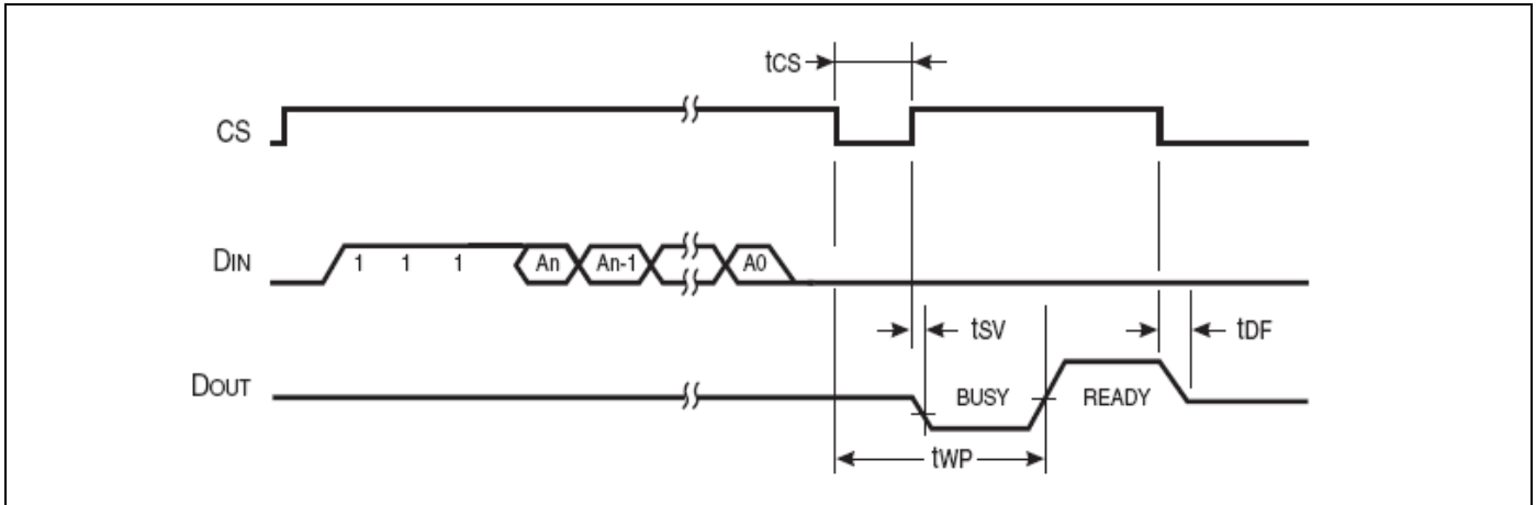
Figure 5.10-7. Erase (Erase) Cycle Timing
