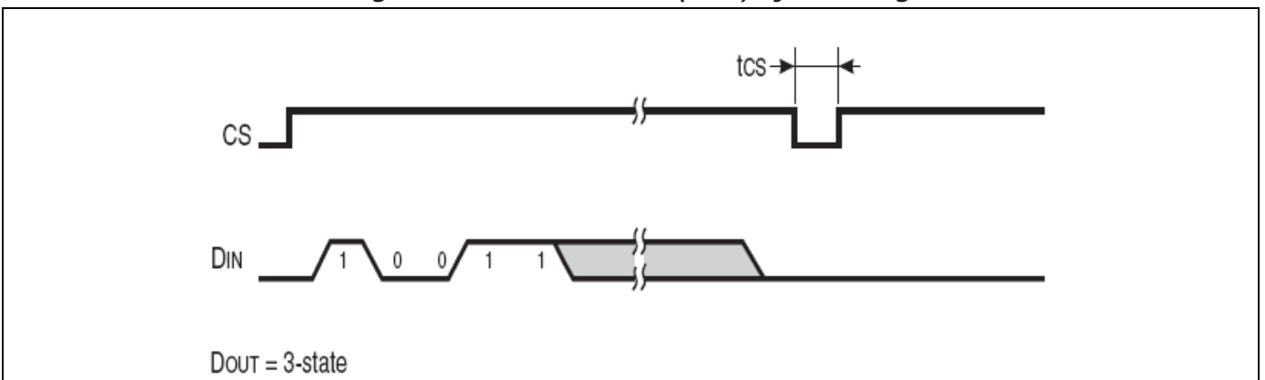
Figure 5.10-3. Write Enable (WEN) Cycle Timing
