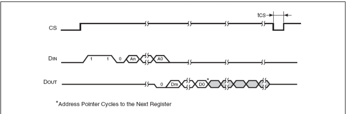
Figure 5.10-2. Read Cycle Timing
