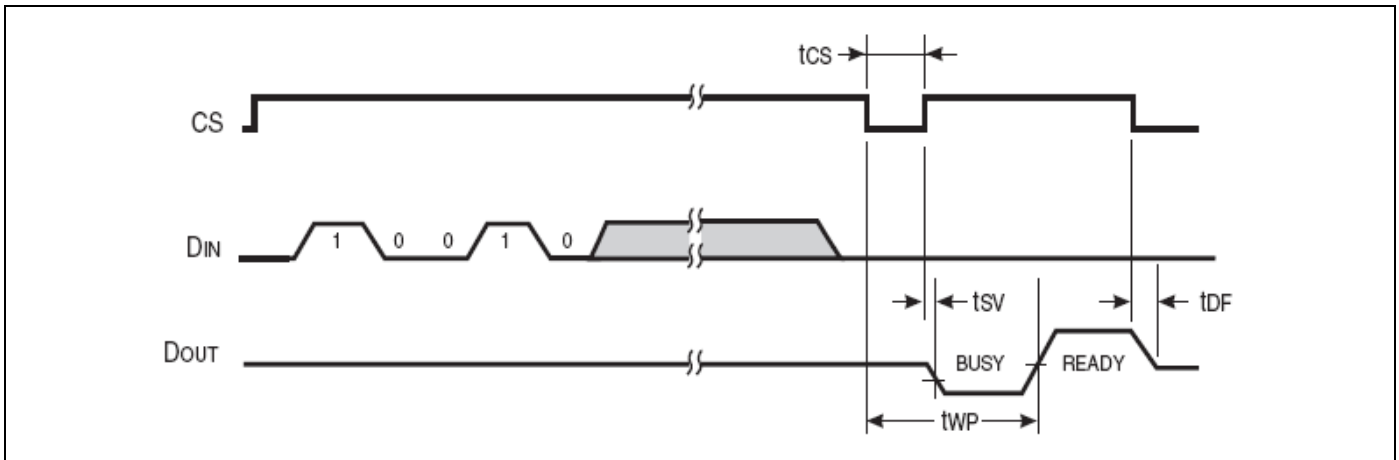
Figure 5.10-8. Erase All (ERAL) Cycle Timing
