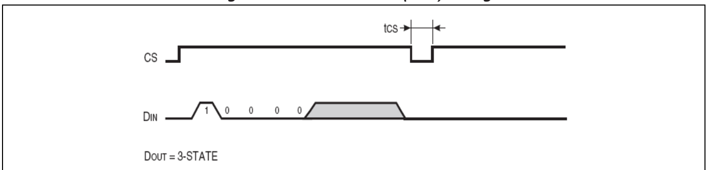
Figure 5.10-6. Write Disable (WDS) Timing
