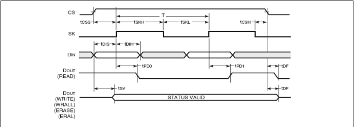
Figure 5.10-1. Synchronous Data Timing
