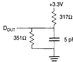
Figure 2. Output Load Equivalent (for t_{LZCE} , t_{HZCE} , t_{LZWE} , t_{HZWE} , t_{LZOE} , t_{HZOE} )
