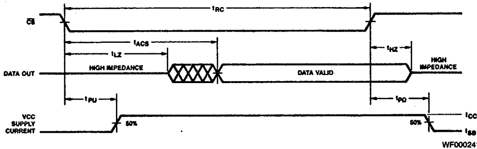
Read Cycle No. 2 (Notes 8, 10)
