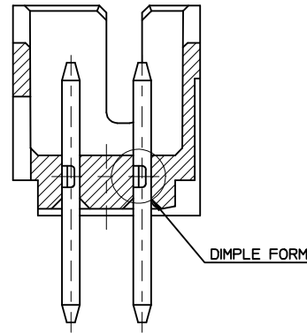
SECTION X-X SCALE 4:1
