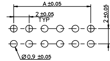
P.C. BOARD LAYOUT (THICKNESS:1.6t)
