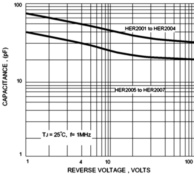
FIG.3 - TYPICAL JUNCTION CAPACITANCE
