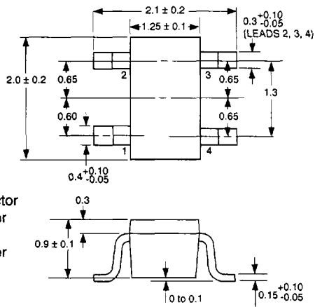
PACKAGE OUTLINE 18 (SOT-343)
