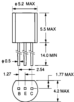
PACKAGE OUTLINE 32 (TO-92)
