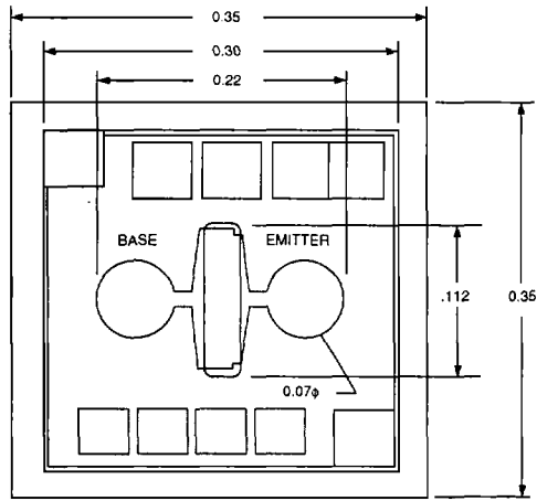
NE85600 (CHIP)
