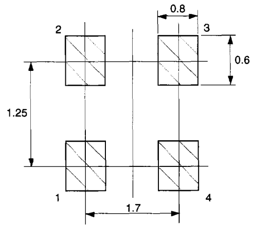
PACKAGE OUTLINE 18 RECOMMENDED P.C.B. LAYOUT
