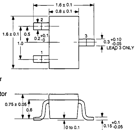
PACKAGE OUTLINE 19
