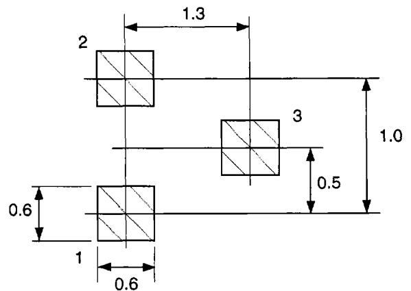
PACKAGE OUTLINE 19 RECOMMENDED P.C.B. LAYOUT
