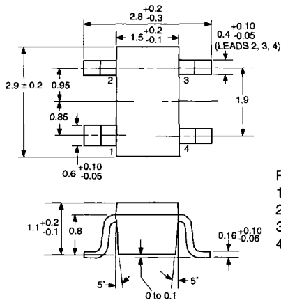
PACKAGE OUTLINE 39
