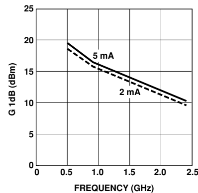
Figure 6. AT-30511 1 dB Compressed Gain vs. Frequency and Current at V_{CE} = 2.7\text{ V} .
