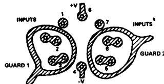
Figure 29. Board Layout for Guarding Inputs
