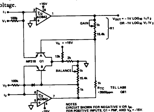
Figure 28. Log-Ratio Amplifier
