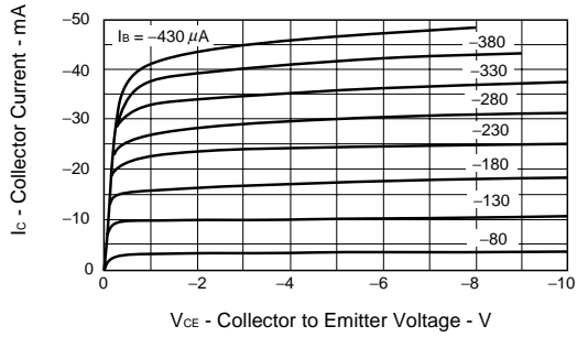
COLLECTOR CURRENT vs. COLLECTOR TO EMITTER VOLTAGE
