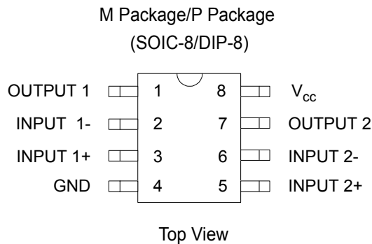
Figure 2. Pin Configuration of HWD358
