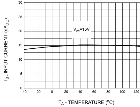
Figure 5. Input Current
