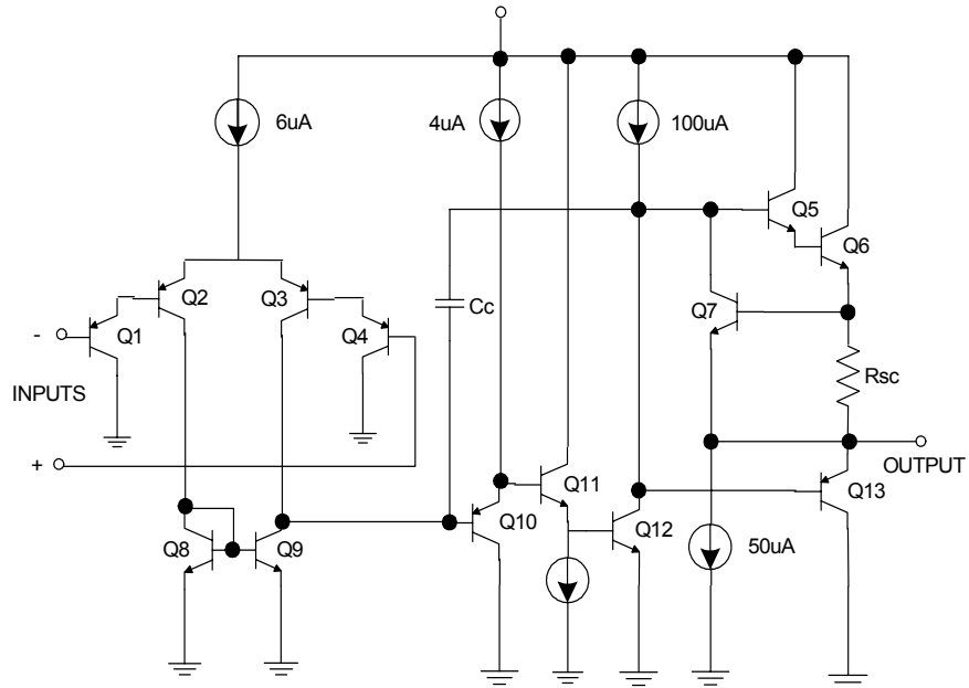
Figure 3. Functional Block Diagram of HWD358 (Each Amplifier)
