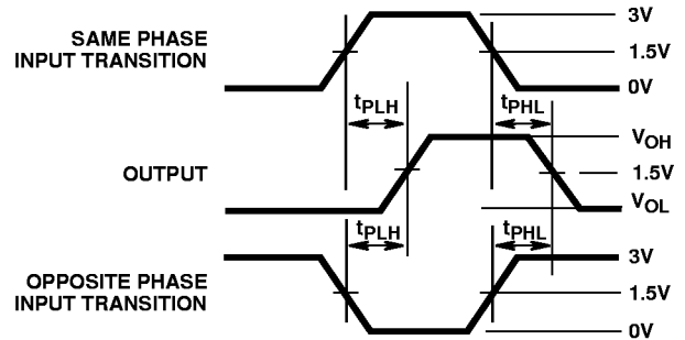
FIGURE 3. PROPAGATION DELAY
