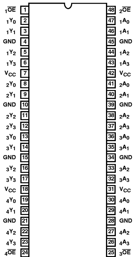
CD74LPT16244 (SSOP, TSSOP) TOP VIEW
