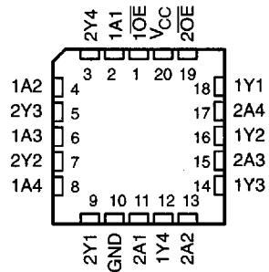
SN54F240 ... FK PACKAGE (TOP VIEW)
