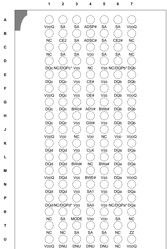
TOP VIEW
