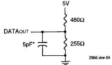
Figure 2. AC Test Load (for t CLZ , t OLZ , t CHZ , t OHZ , t LOW , and t WHZ )
