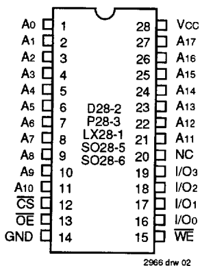
DIP/SOJ/LCC TOP VIEW
