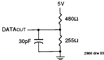
Figure 1. AC Test Load
