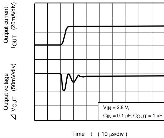
TCR5SC18FE ( I_{OUT} = 1\text{m to }30\text{mA} )
