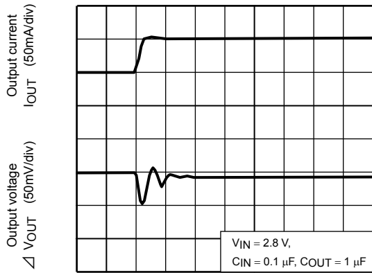
TCR5SC18FE ( I_{OUT} = 50\text{m to }100\text{mA} )
