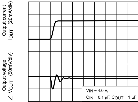
TCR5SC30FE ( I_{OUT} = 1\text{m to }30\text{mA} )
