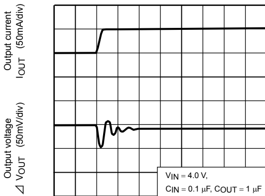
TCR5SC30FE ( I_{OUT} = 50\text{m to }100\text{mA} )
