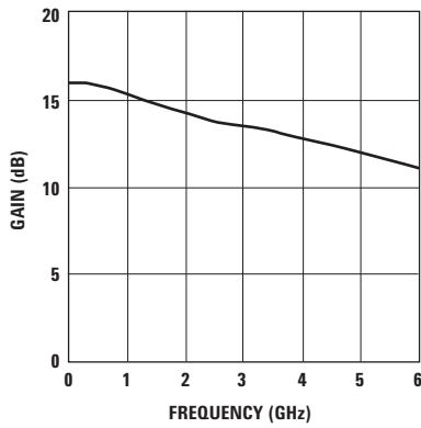
Figure 3. Gain vs. Frequency at I_d = 15 \text{ mA} .
