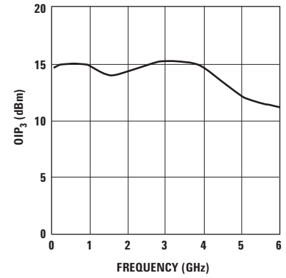
Figure 5. OIP_3 vs. Frequency at I_d = 15 \text{ mA} .
