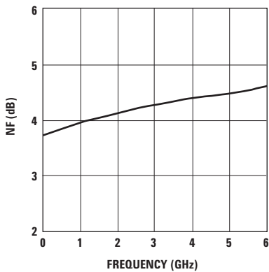
Figure 6. NF vs Frequency at I_d = 15 \text{ mA} .
