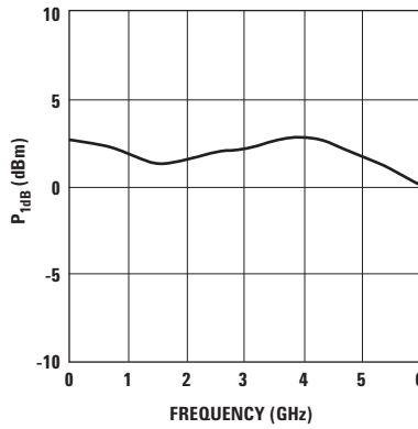
Figure 4. P_{1dB} vs. Frequency at I_d = 15 \text{ mA} .
