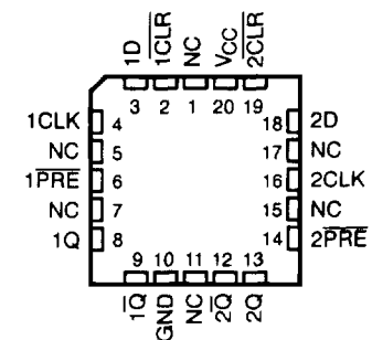
SN54AHCT74 ... FK PACKAGE (TOP VIEW)
