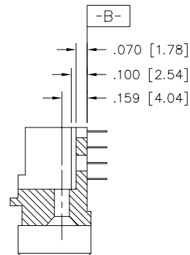
SECTION W-W
