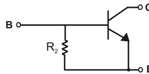
SCHMATIC DIAGRAM
