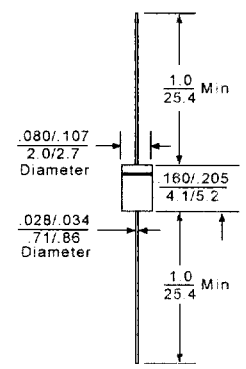
DO-41
