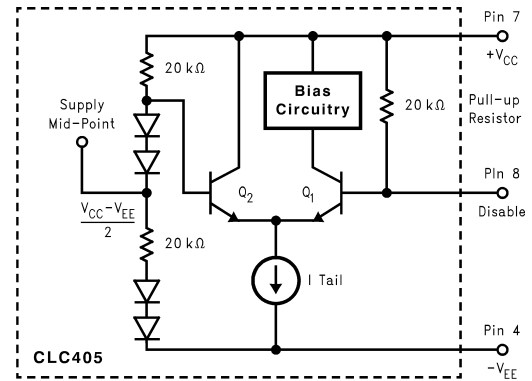
FIGURE 1. Enable/Disable Operation for Single or Unbalanced Supply Operation
