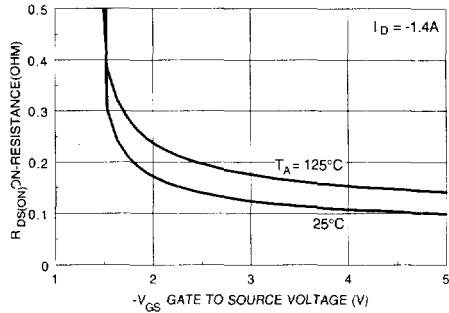
Figure 4. On-Resistance Variation with Gate-To-Source Voltage.
