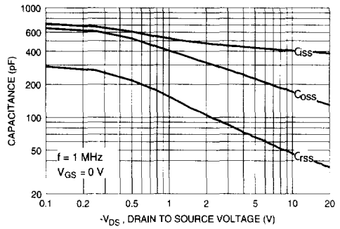
Figure 8. Capacitance Characteristics.
