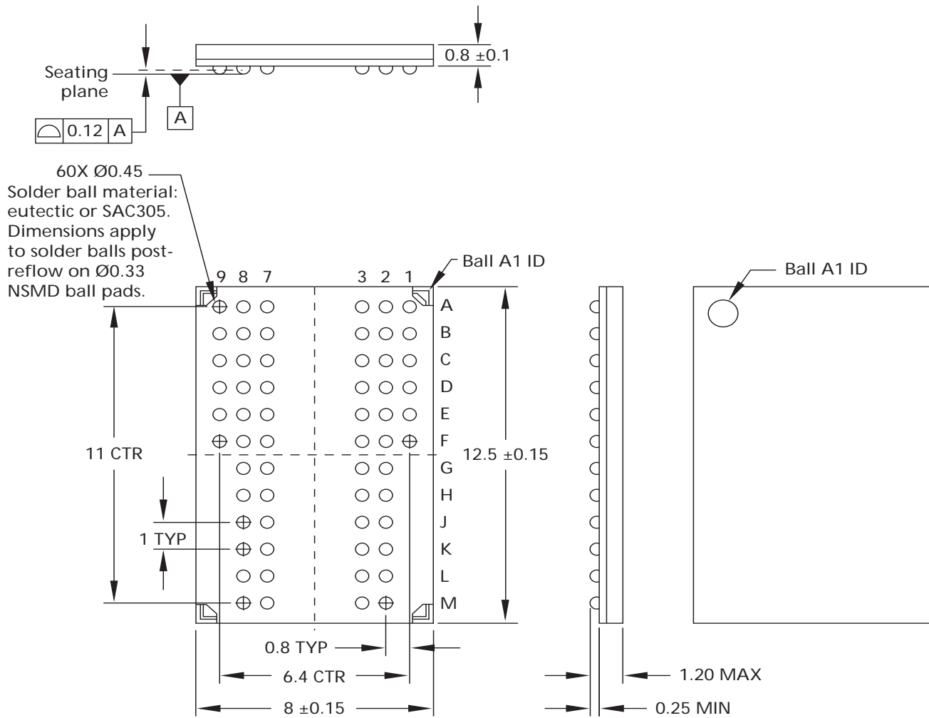
Figure 7: 60-Ball FBGA (8mm x 12.5mm)
