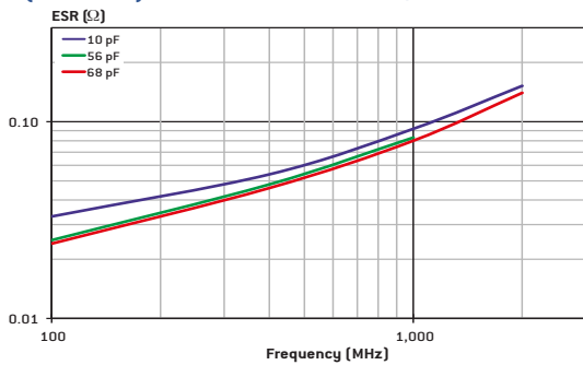
SHS (SIZE 0603): TYPICAL ESR VERSUS FREQUENCY
