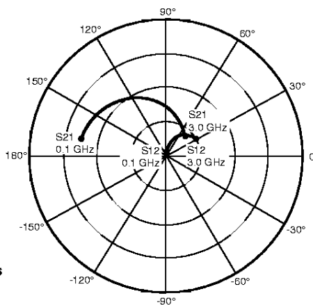
Coordinates in Ohms Frequency in GHz V CE = 2.5 V, I c = 1 mA Z 0 = 50 Ω
