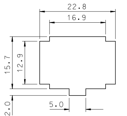
PANEL HOLE DIMENSION
