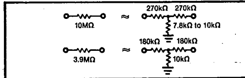
FIGURE 4. Equivalent Resistances.
