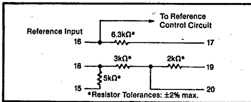
FIGURE 7. Internal Scaling Resistors.
