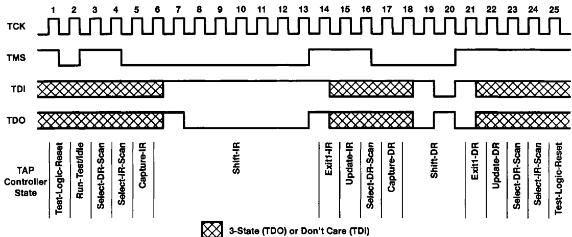
Figure 12. Timing Example
