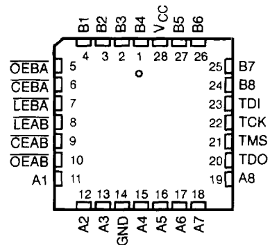
SN54ABT8543 ... FK PACKAGE (TOP VIEW)
