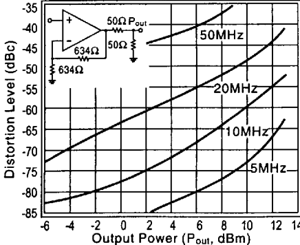
3rd Harmonic Distortion vs. P_out
