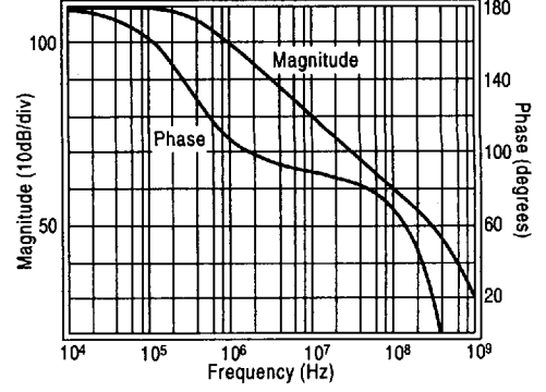
Differential Gain vs. Frequency
