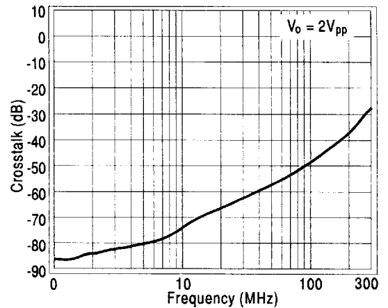
Channel-to-Channel Crosstalk
