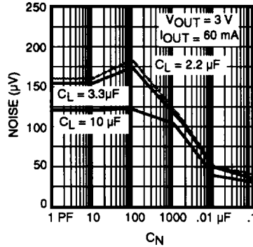
NOISE LEVEL vs. CN
