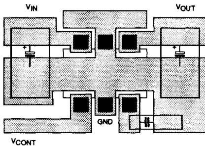
SOT-23L BOARD LAYOUT
