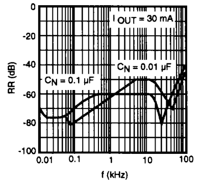
RIPPLE REJECTION
