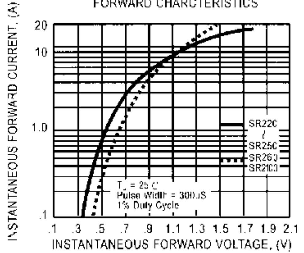
FIG. 2 - TYPICAL INSTANTANEOUS FORWARD CHARACTERISTICS
