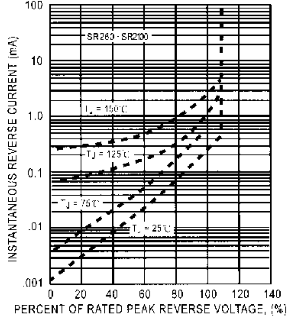
FIG. 3B - TYPICAL REVERSE CHARACTERISTICS
