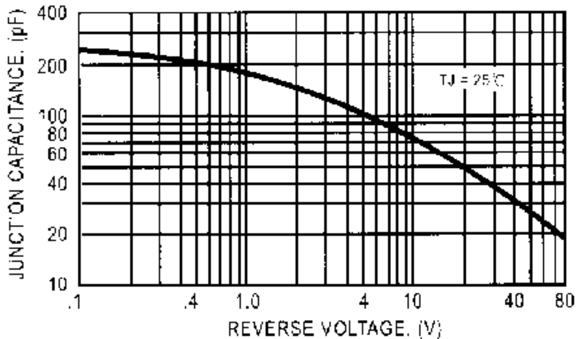
FIG. 4 - TYPICAL JUNCTION CAPACITANCE
