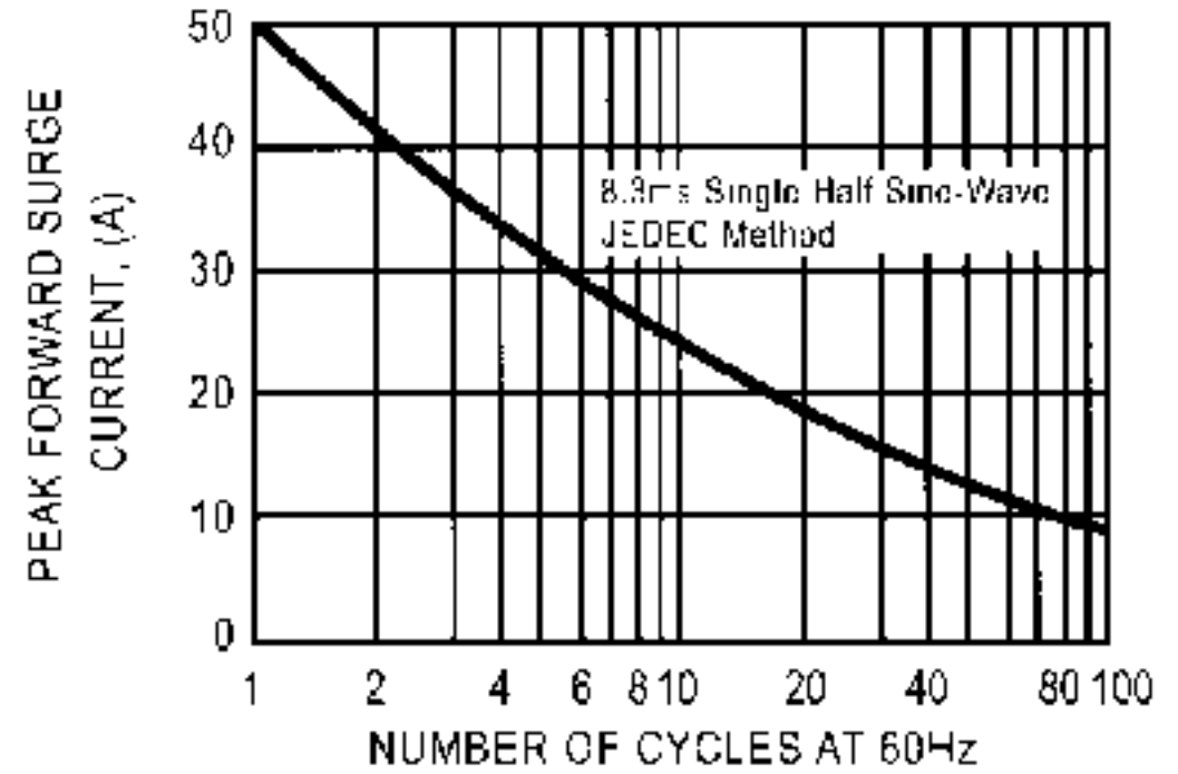
FIG. 5 - MAXIMUM NON-REPETITIVE FORWARD SURGE CURRENT
