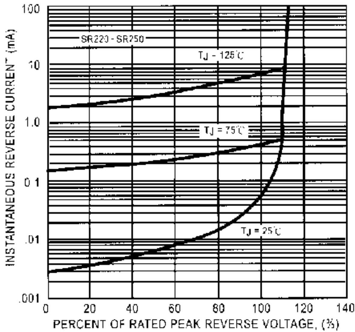
FIG. 3A - TYPICAL REVERSE CHARACTERISTICS
