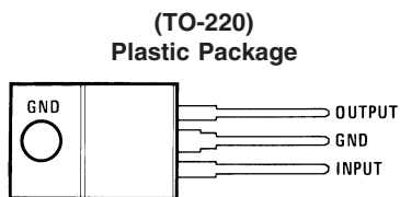
Front View Order Number LM2930T-5.0 or LM2930T-8.0 See NS Package Number T03B
