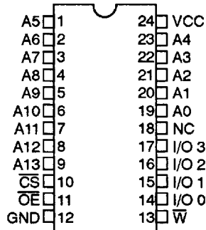
Pinout 24 pins (top view)
