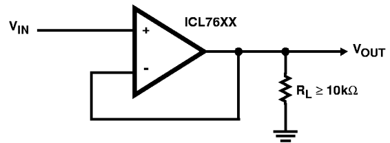
FIGURE 1. SIMPLE FOLLOWER
