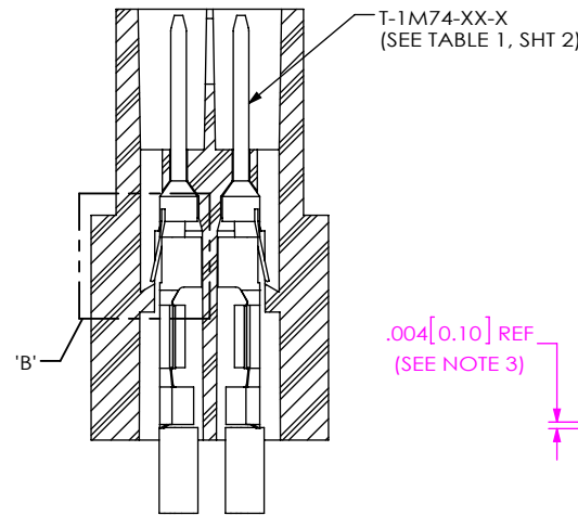
SECTION "A"- "A" SCALE 3 : 1
